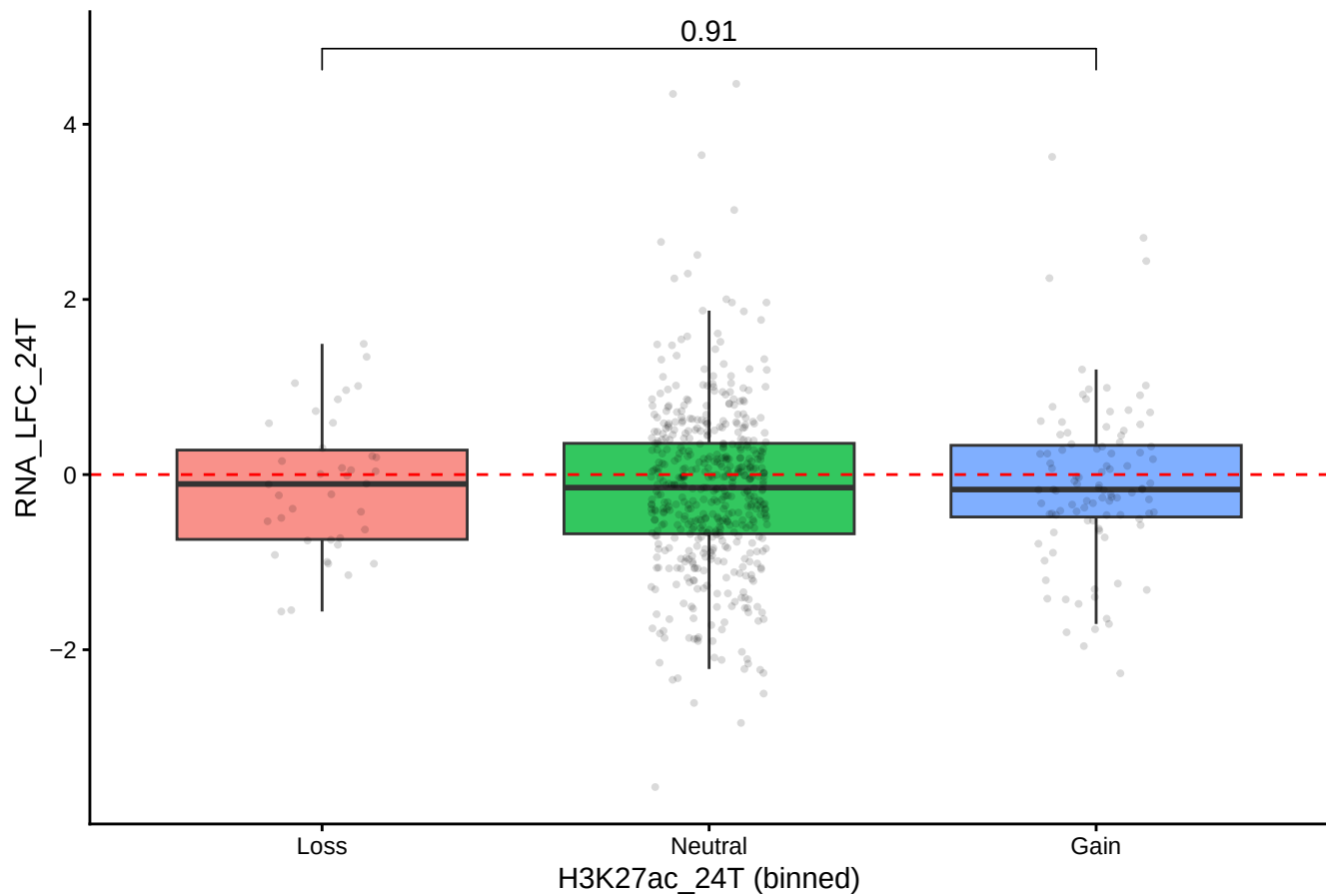
RNA_LFC_24T by H3K27ac_24T - Set_1
